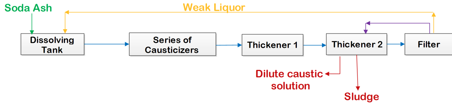
Figure: Manufacturing of Caustic Soda by Lime Soda Process
